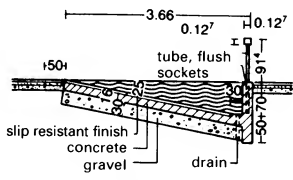
5 Steeplechase water jump: section
